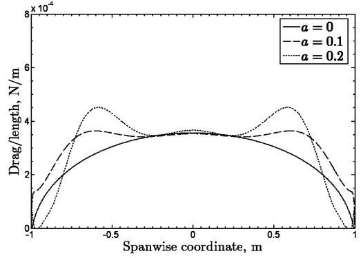
Fig. 7 Drag per unit length distribution of several gull wings, \Lambda = 10 , \alpha = 3 deg.
